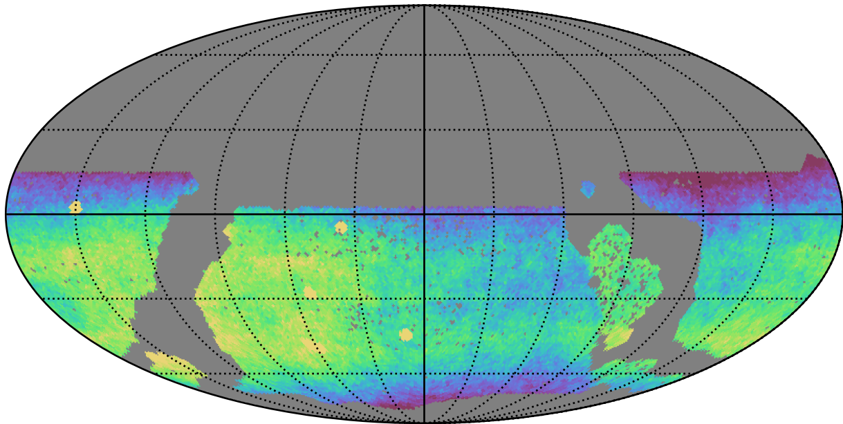
baseline_v3.3_10yrs WFD r band: CoaddM5
