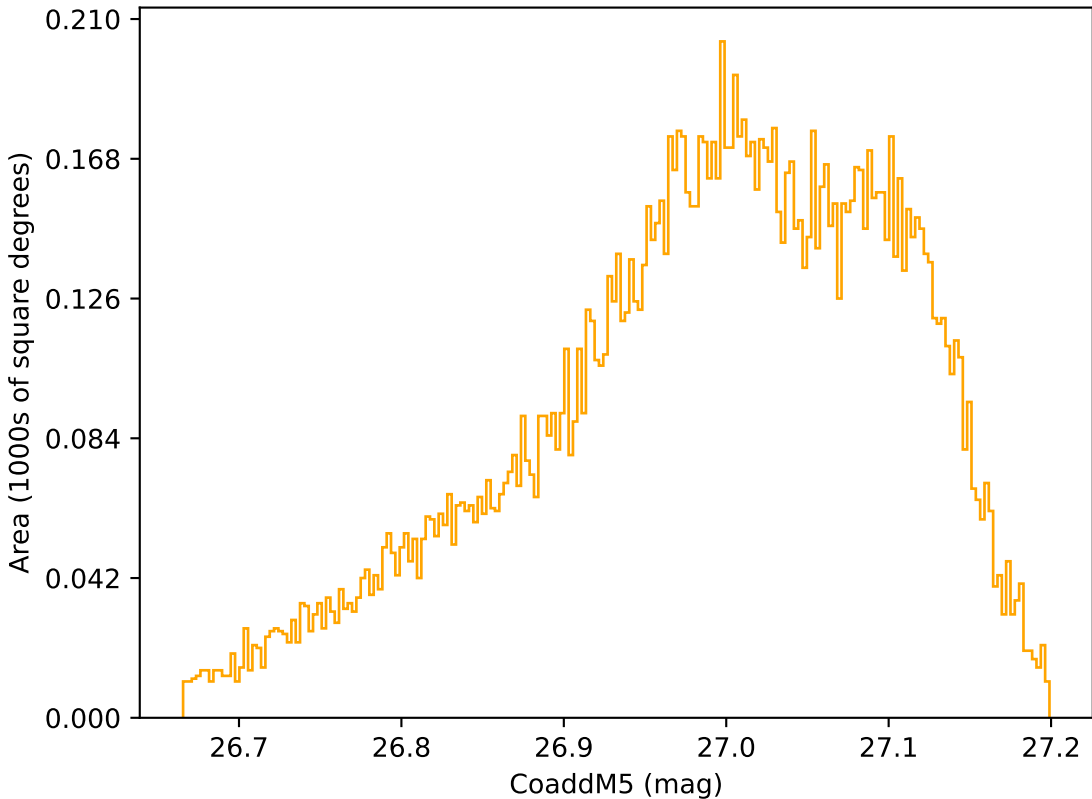
baseline_v3.3_10yrs WFD r band: CoaddM5
