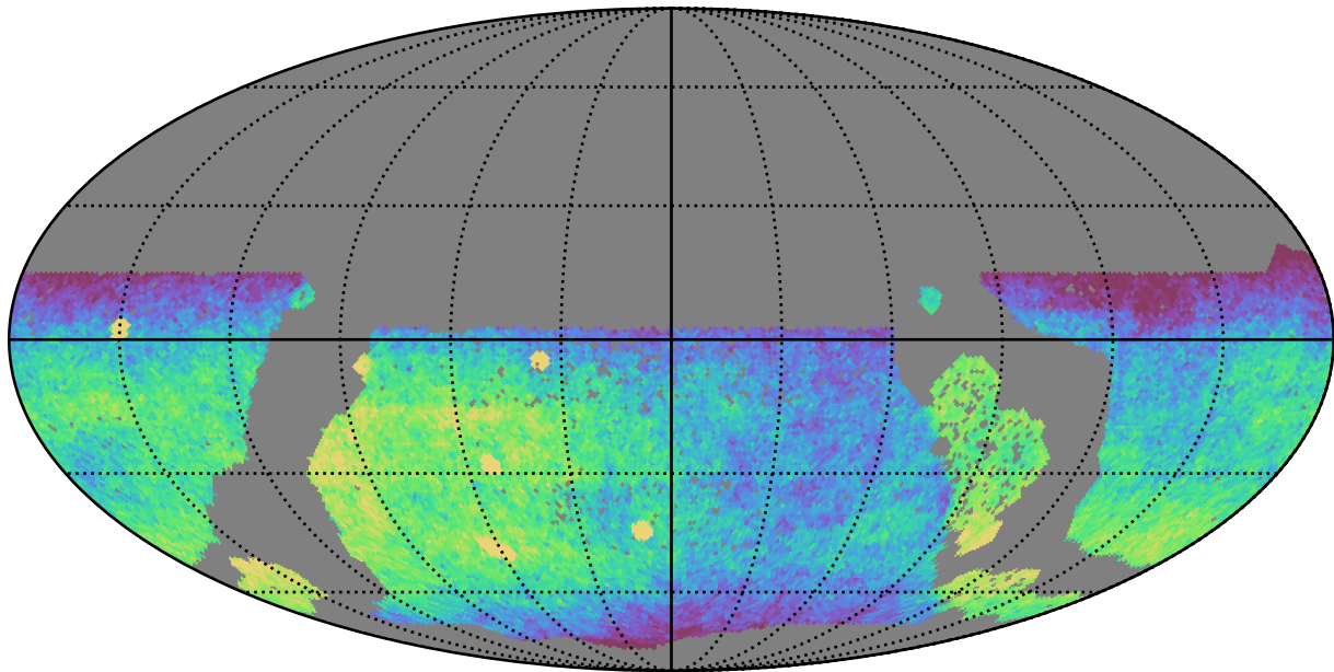
baseline_v3.3_10yrs WFD g band: CoaddM5
