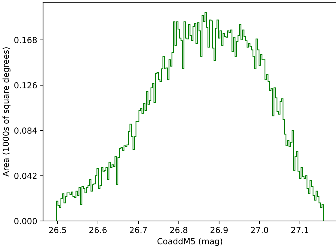
baseline_v3.3_10yrs WFD g band: CoaddM5
