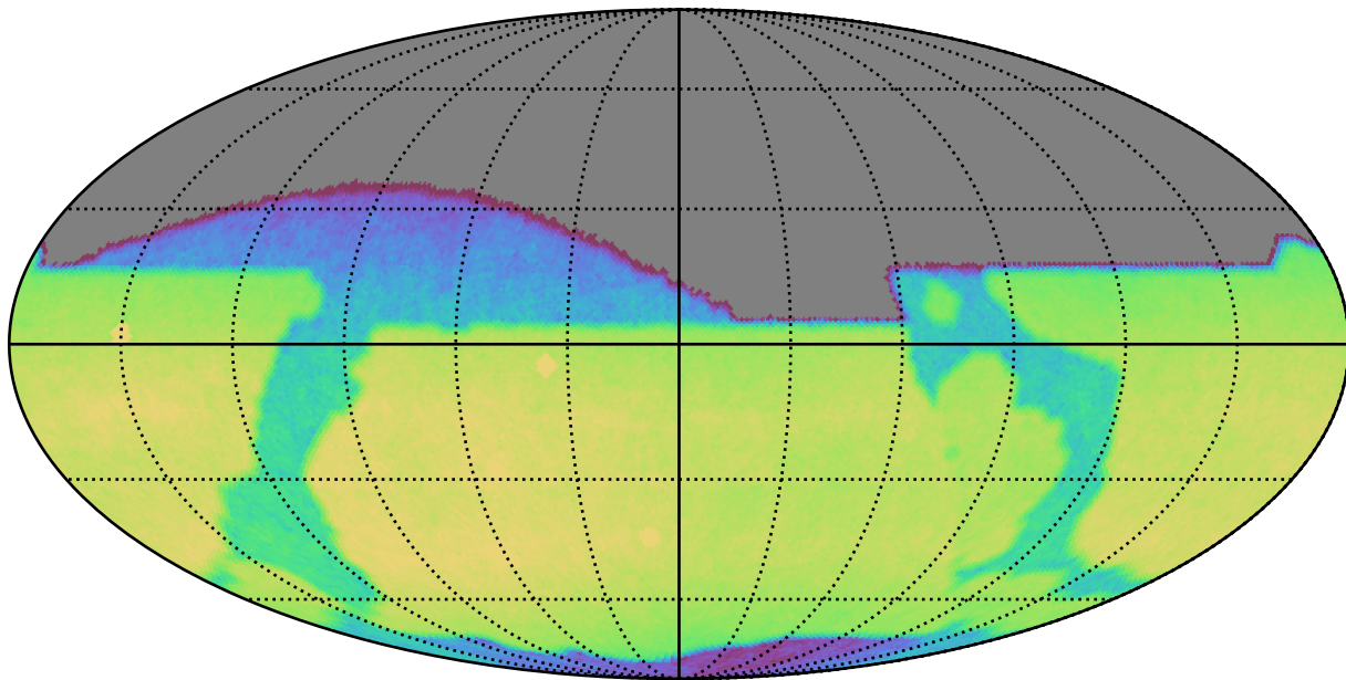
baseline_v3.3_10yrs All sky z band: CoaddM5
