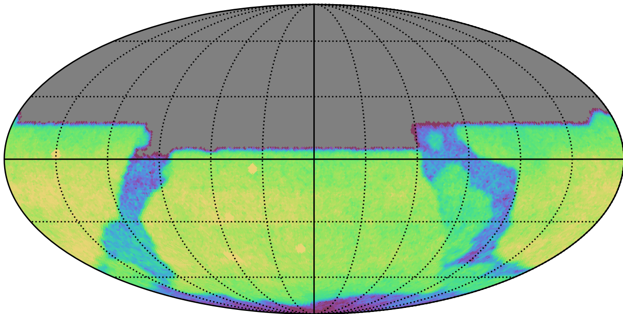
baseline_v3.3_10yrs All sky u band: CoaddM5
