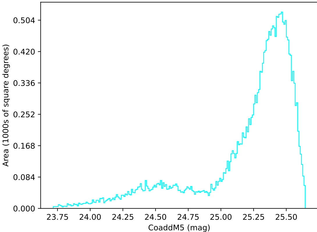
baseline_v3.3_10yrs All sky u band: CoaddM5
