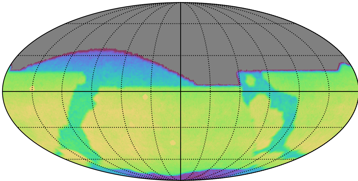
baseline_v3.3_10yrs All sky r band: CoaddM5
