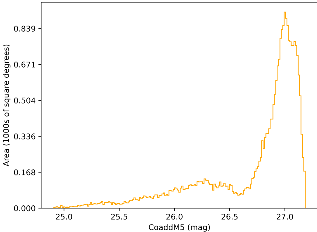
baseline_v3.3_10yrs All sky r band: CoaddM5
