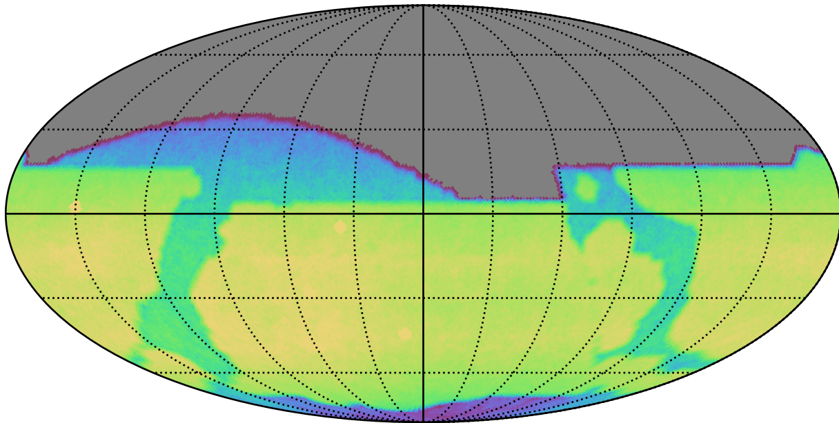
baseline_v3.3_10yrs All sky i band: CoaddM5
