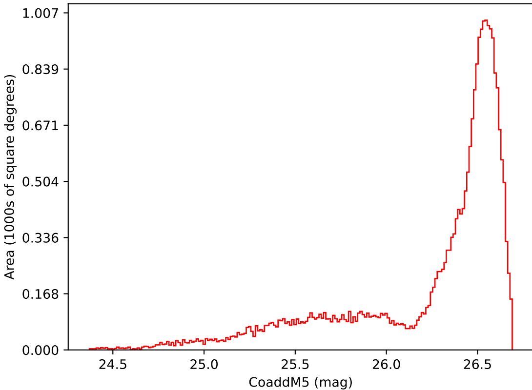
baseline_v3.3_10yrs All sky i band: CoaddM5
