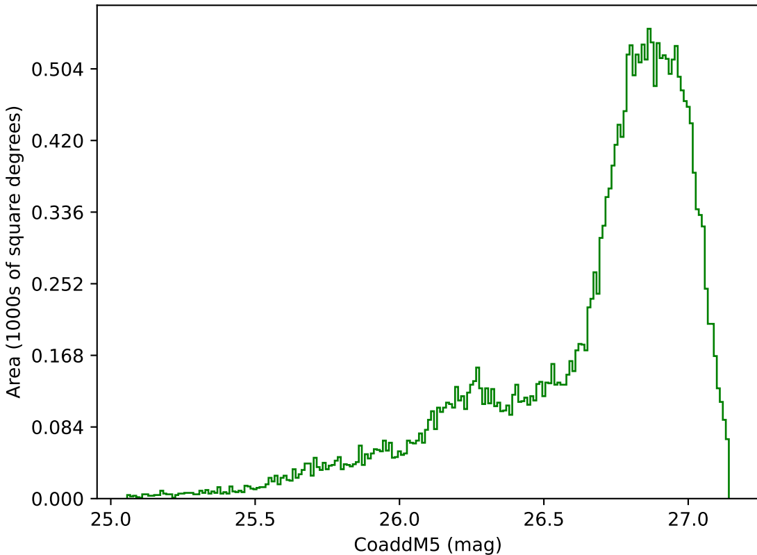
baseline_v3.3_10yrs All sky g band: CoaddM5
