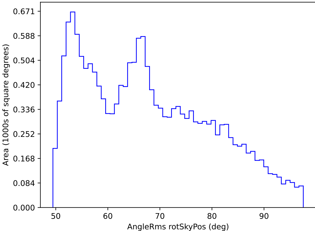
baseline_v3.3_10yrs WFD all bands: AngleRms rotSkyPos
