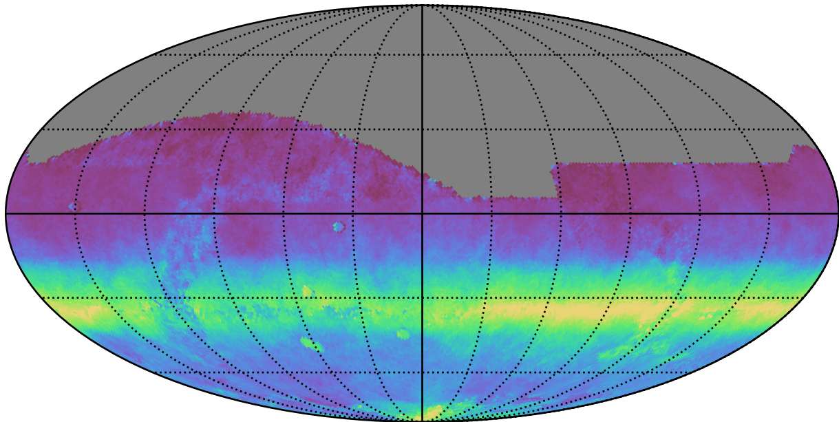
baseline_v3.3_10yrs All sky all bands: AngleRms rotSkyPos
