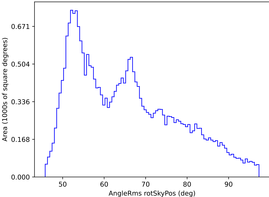
baseline_v3.3_10yrs All sky all bands: AngleRms rotSkyPos
