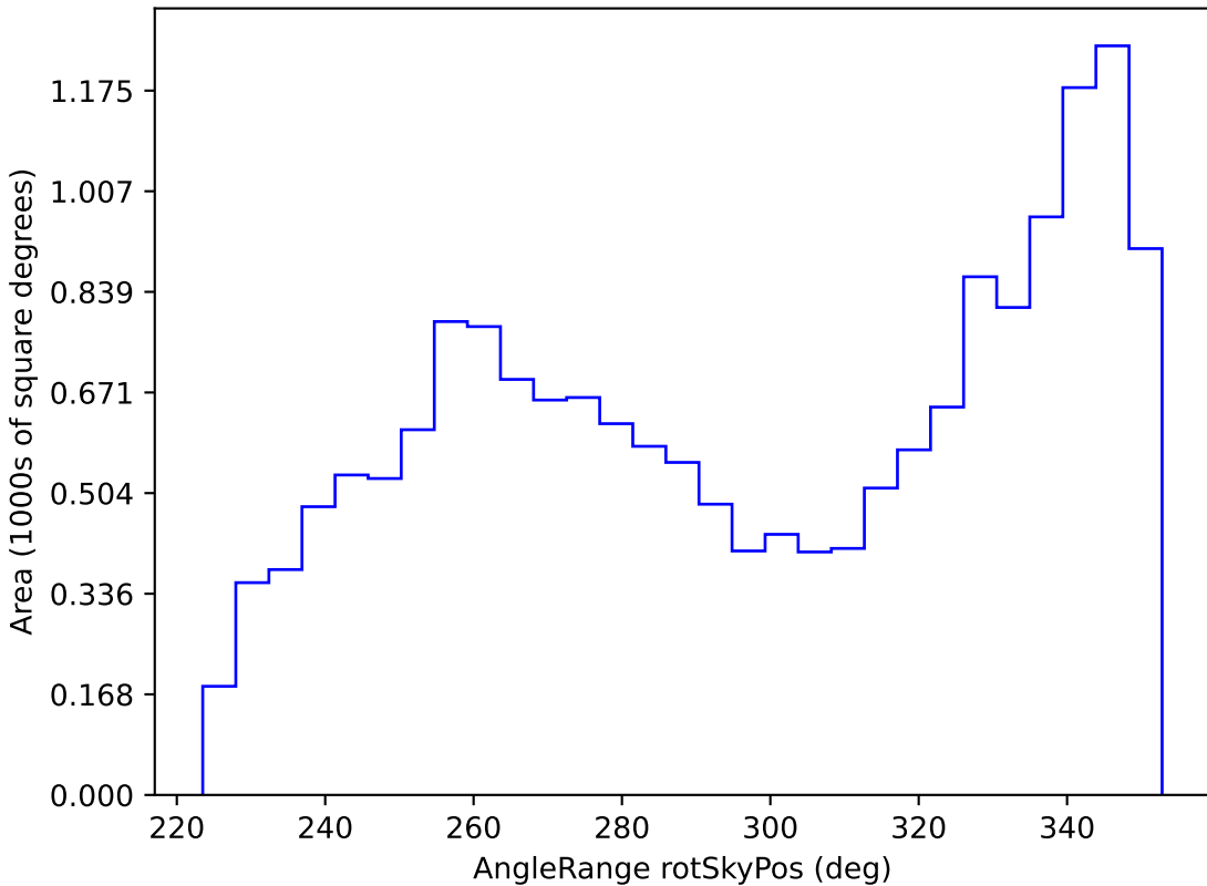
baseline_v3.3_10yrs WFD all bands: AngleRange rotSkyPos
