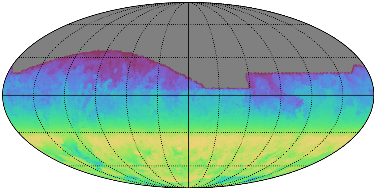
baseline_v3.3_10yrs All sky all bands: AngleRange rotSkyPos
