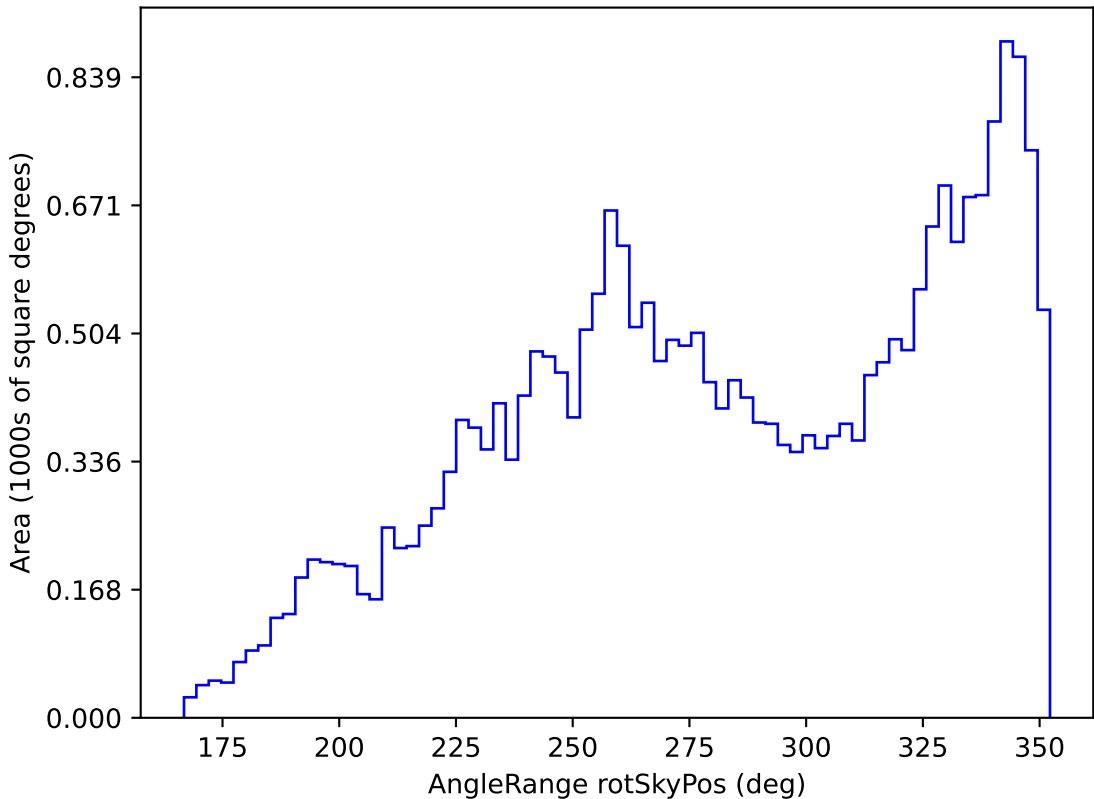
baseline_v3.3_10yrs All sky all bands: AngleRange rotSkyPos
