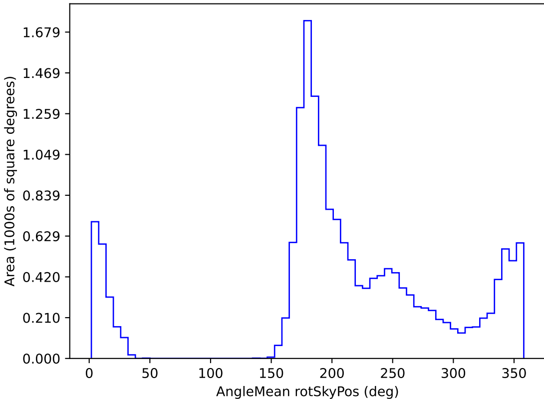
baseline_v3.3_10yrs WFD z band: AngleMean rotSkyPos
