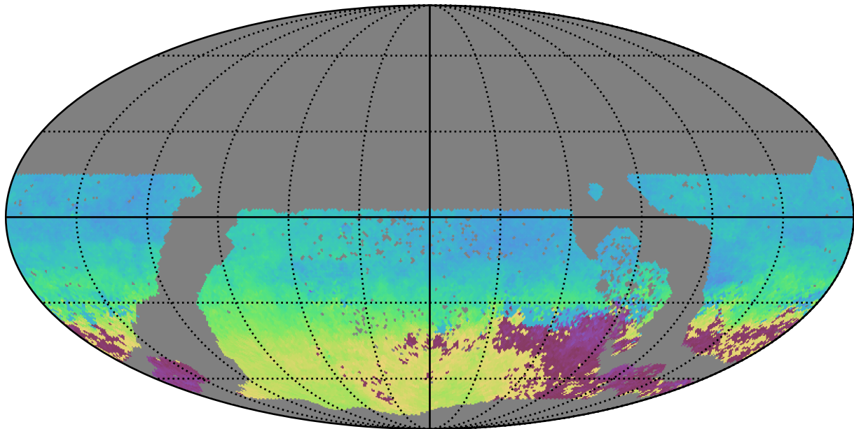
baseline_v3.3_10yrs WFD u band: AngleMean rotSkyPos
