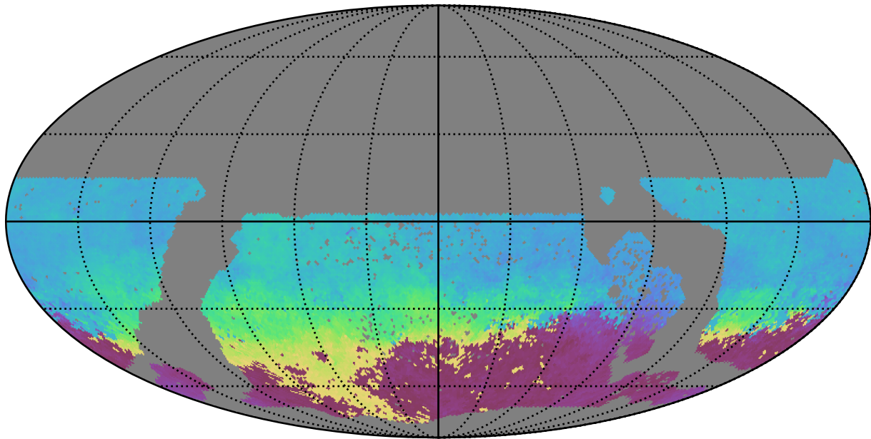
baseline_v3.3_10yrs WFD g band: AngleMean rotSkyPos
