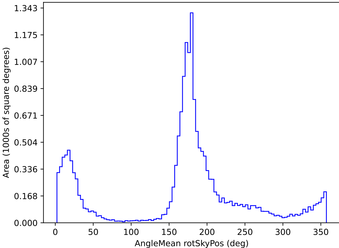
baseline_v3.3_10yrs WFD g band: AngleMean rotSkyPos
