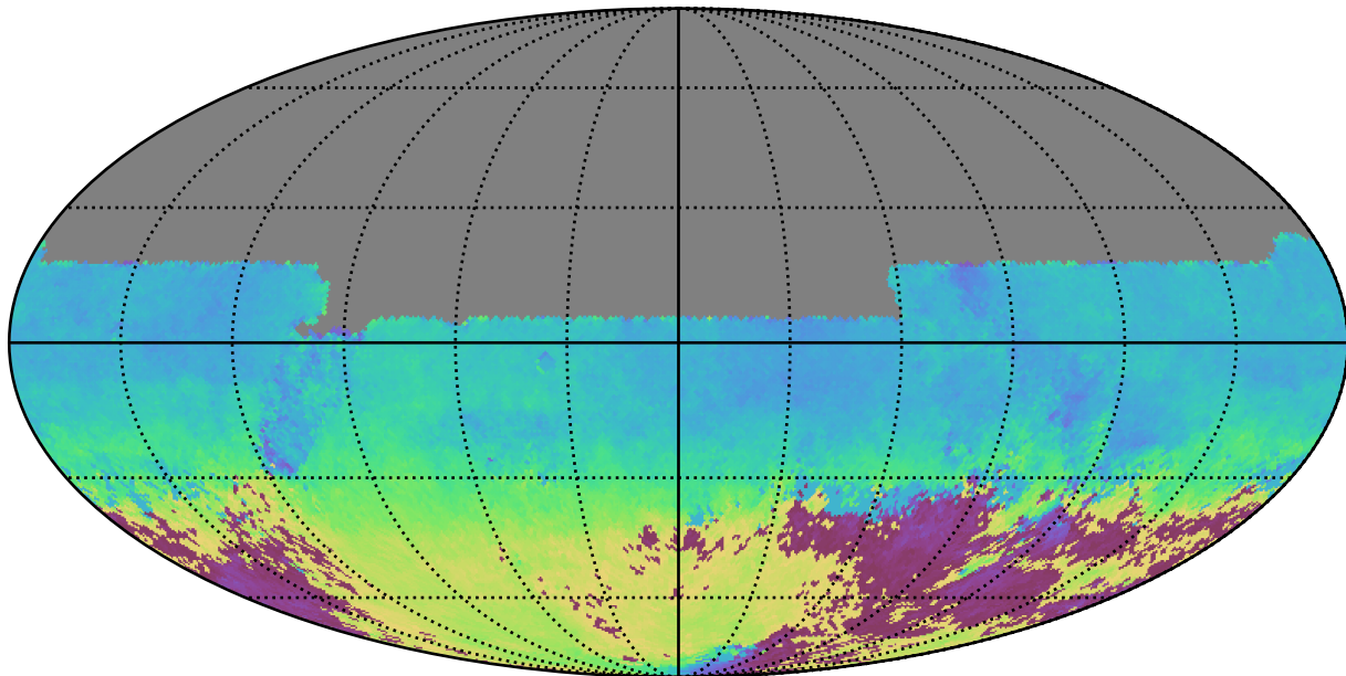
baseline_v3.3_10yrs All sky u band: AngleMean rotSkyPos
