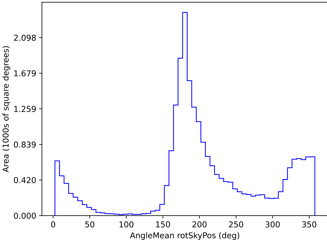
baseline_v3.3_10yrs All sky u band: AngleMean rotSkyPos
