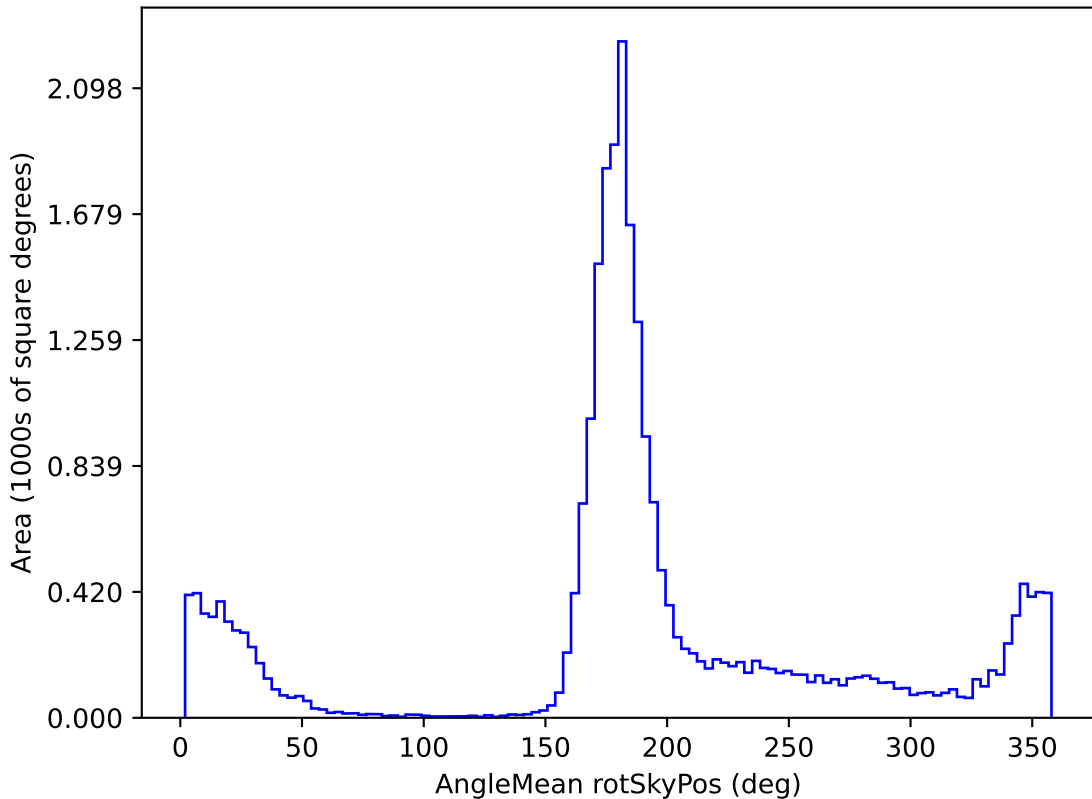
baseline_v3.3_10yrs All sky r band: AngleMean rotSkyPos
