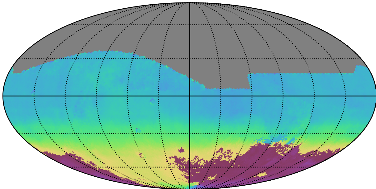
baseline_v3.3_10yrs All sky all bands: AngleMean rotSkyPos
