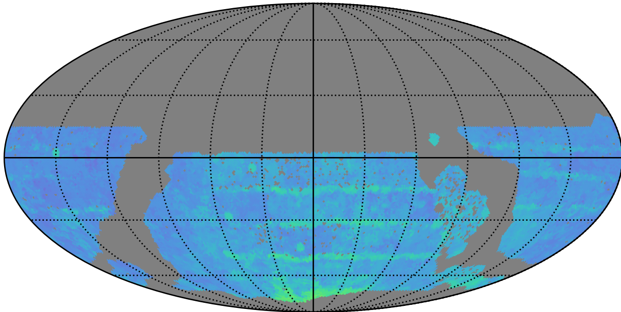
baseline_v3.3_10yrs WFD z band: 80thPercentile Season Length
