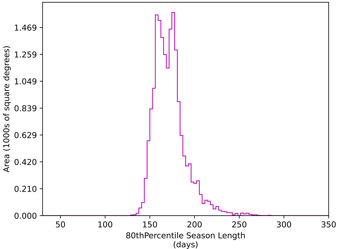
baseline_v3.3_10yrs WFD z band: 80thPercentile Season Length
