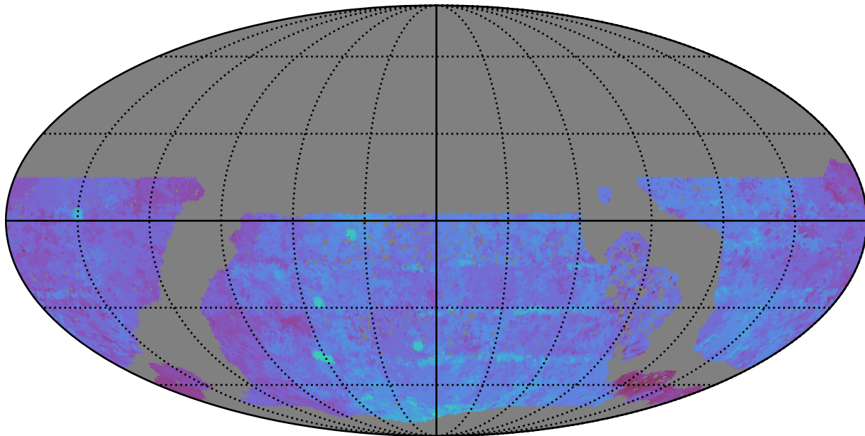
baseline_v3.3_10yrs WFD u band: 80thPercentile Season Length
