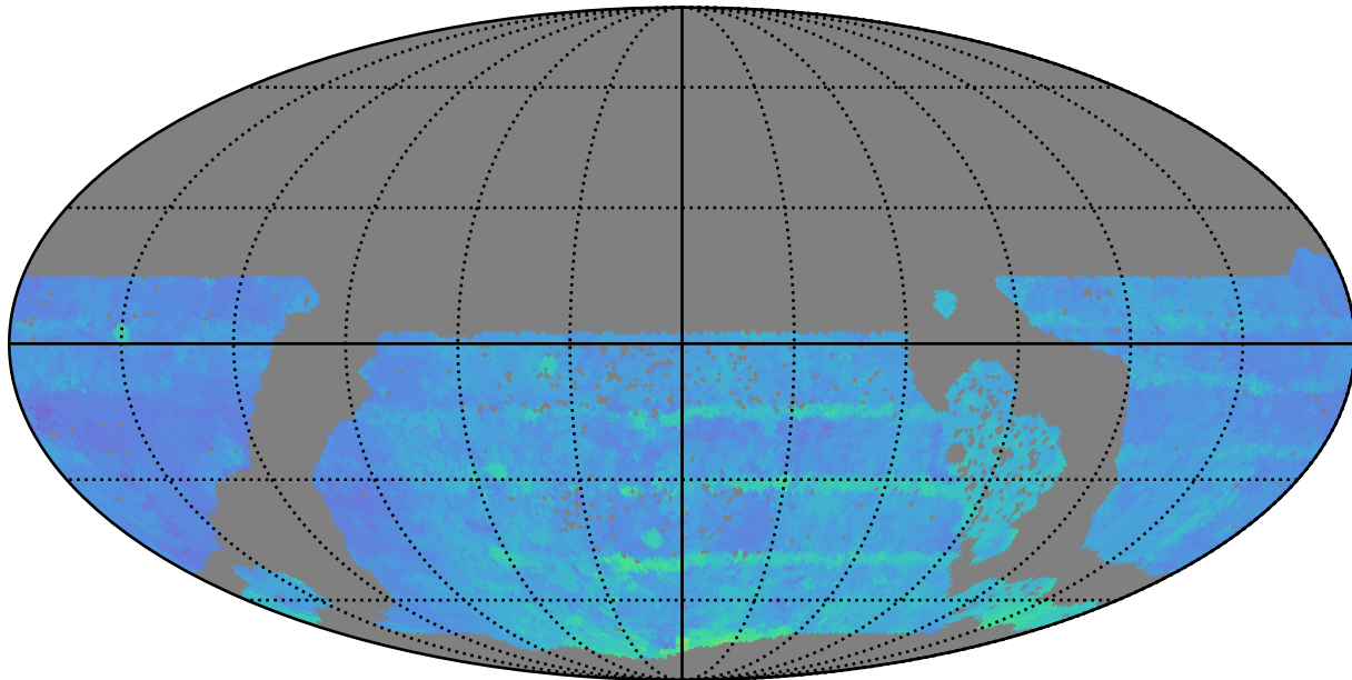
baseline_v3.3_10yrs WFD r band: 80thPercentile Season Length
