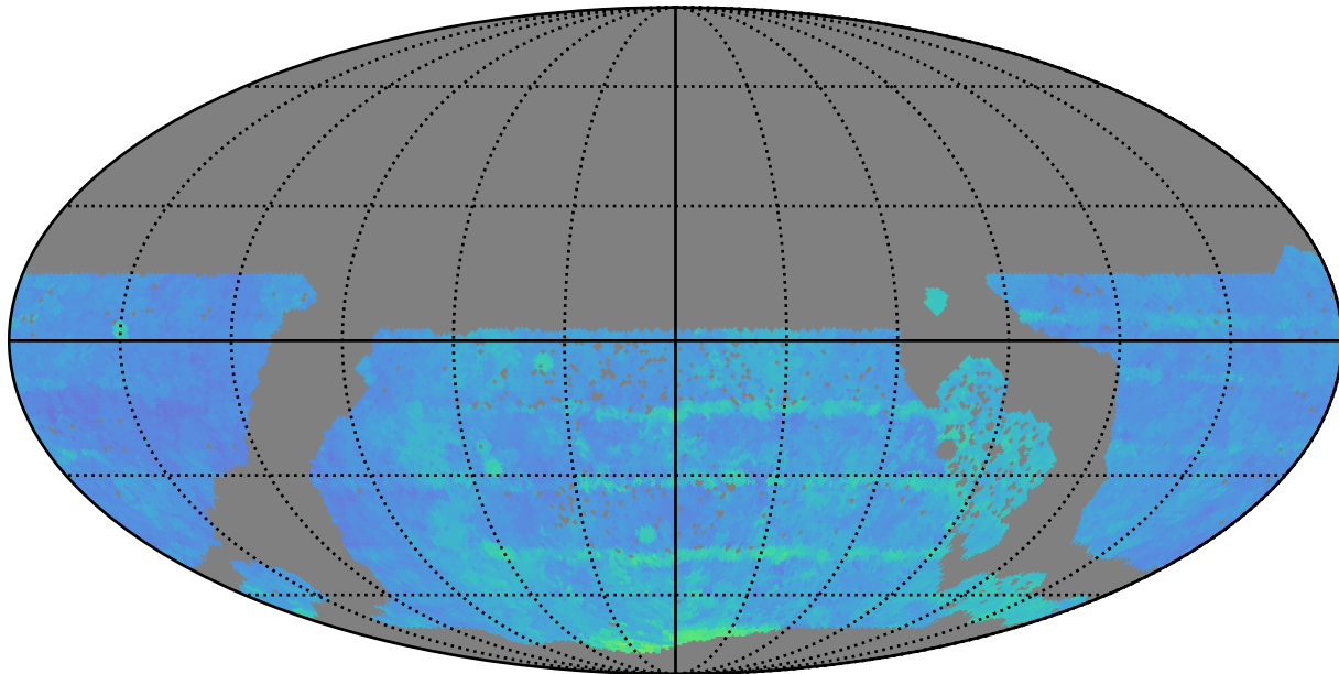
baseline_v3.3_10yrs WFD i band: 80thPercentile Season Length
