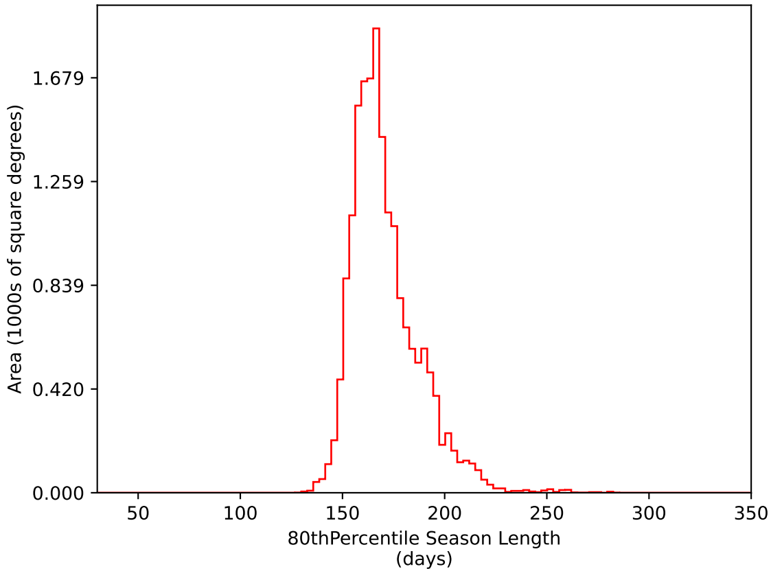
baseline_v3.3_10yrs WFD i band: 80thPercentile Season Length
