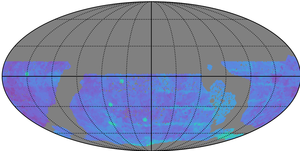
baseline_v3.3_10yrs WFD g band: 80thPercentile Season Length
