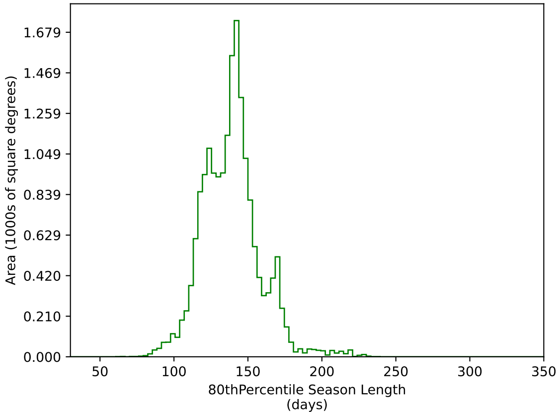
baseline_v3.3_10yrs WFD g band: 80thPercentile Season Length
