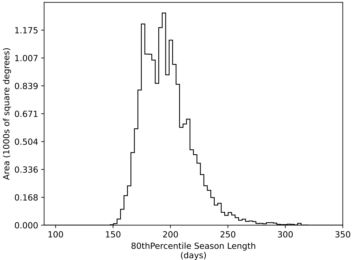
baseline_v3.3_10yrs WFD all bands: 80thPercentile Season Length
