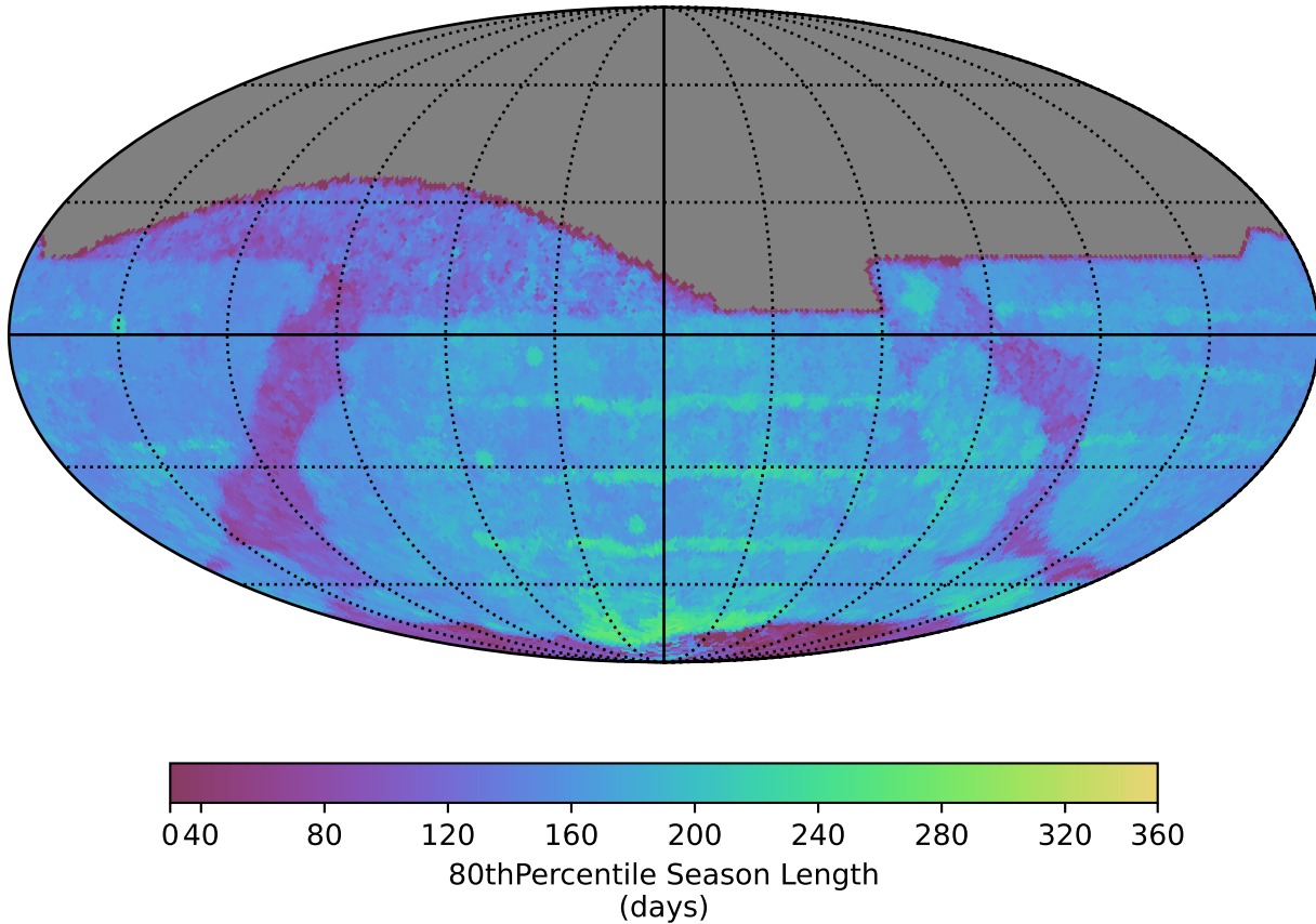
baseline_v3.3_10yrs All sky z band: 80thPercentile Season Length
