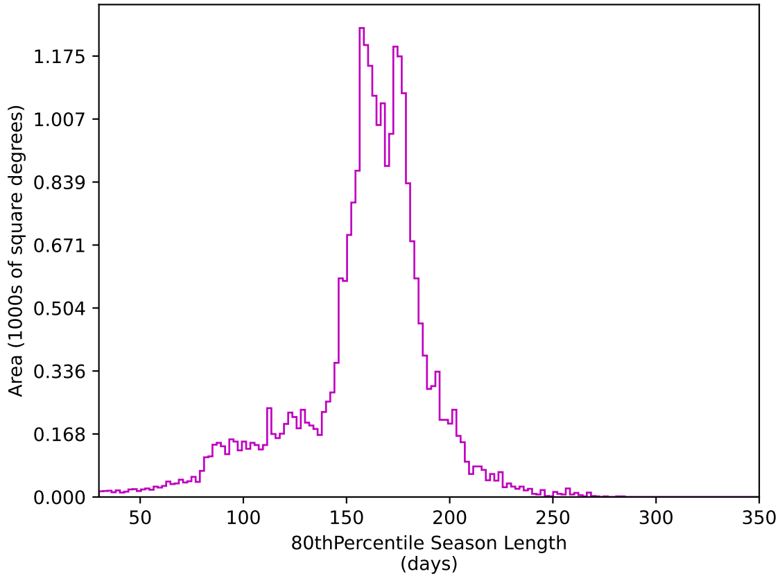
baseline_v3.3_10yrs All sky z band: 80thPercentile Season Length
