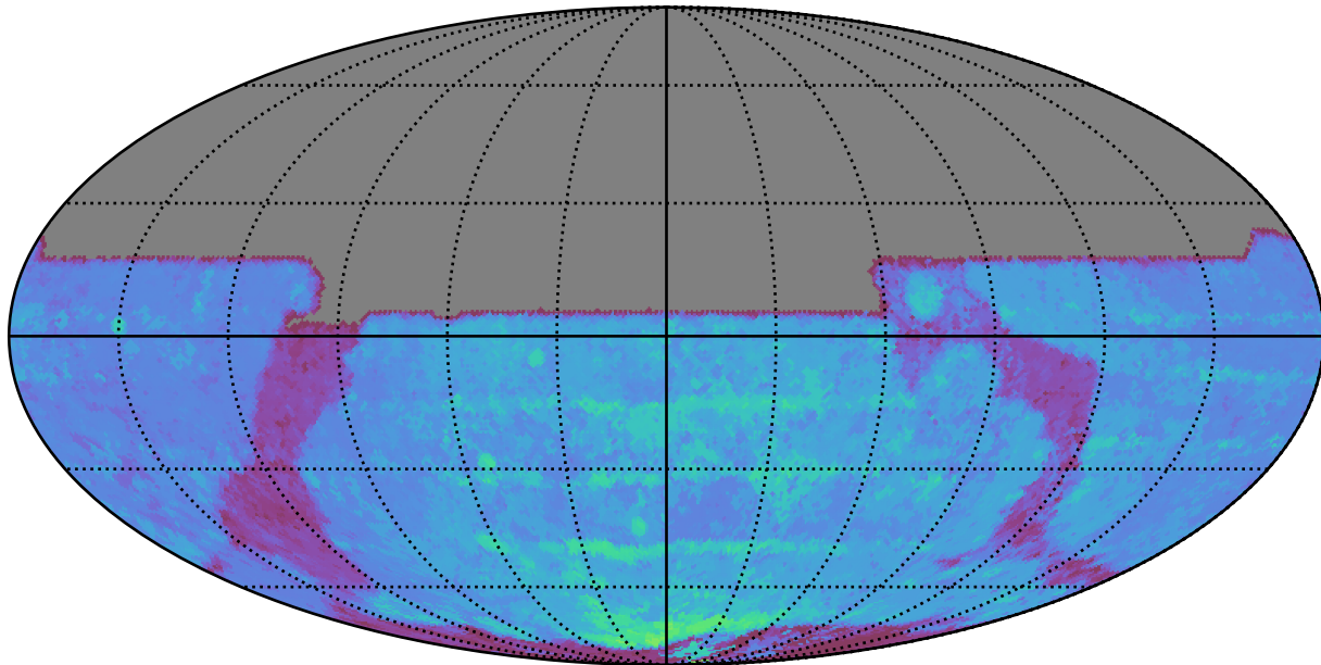
baseline_v3.3_10yrs All sky y band: 80thPercentile Season Length
