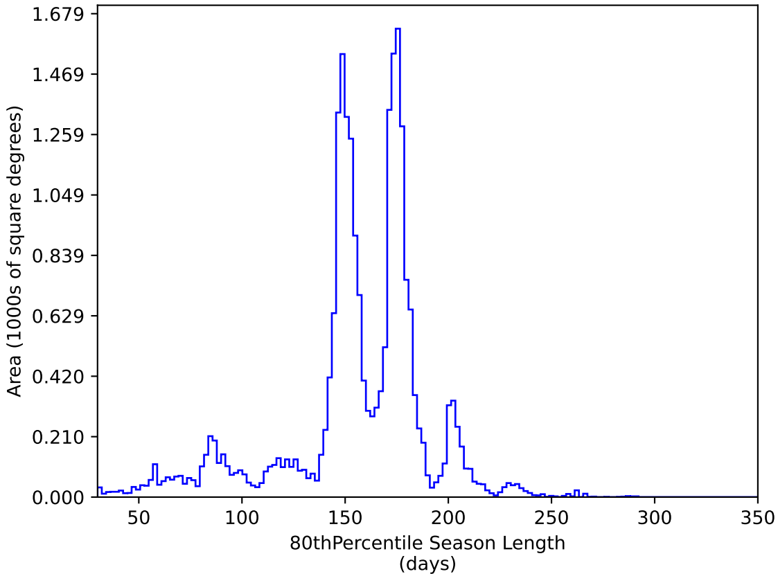
baseline_v3.3_10yrs All sky y band: 80thPercentile Season Length
