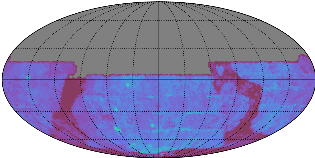
baseline_v3.3_10yrs All sky u band: 80thPercentile Season Length
