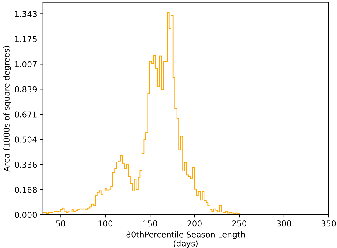
baseline_v3.3_10yrs All sky r band: 80thPercentile Season Length
