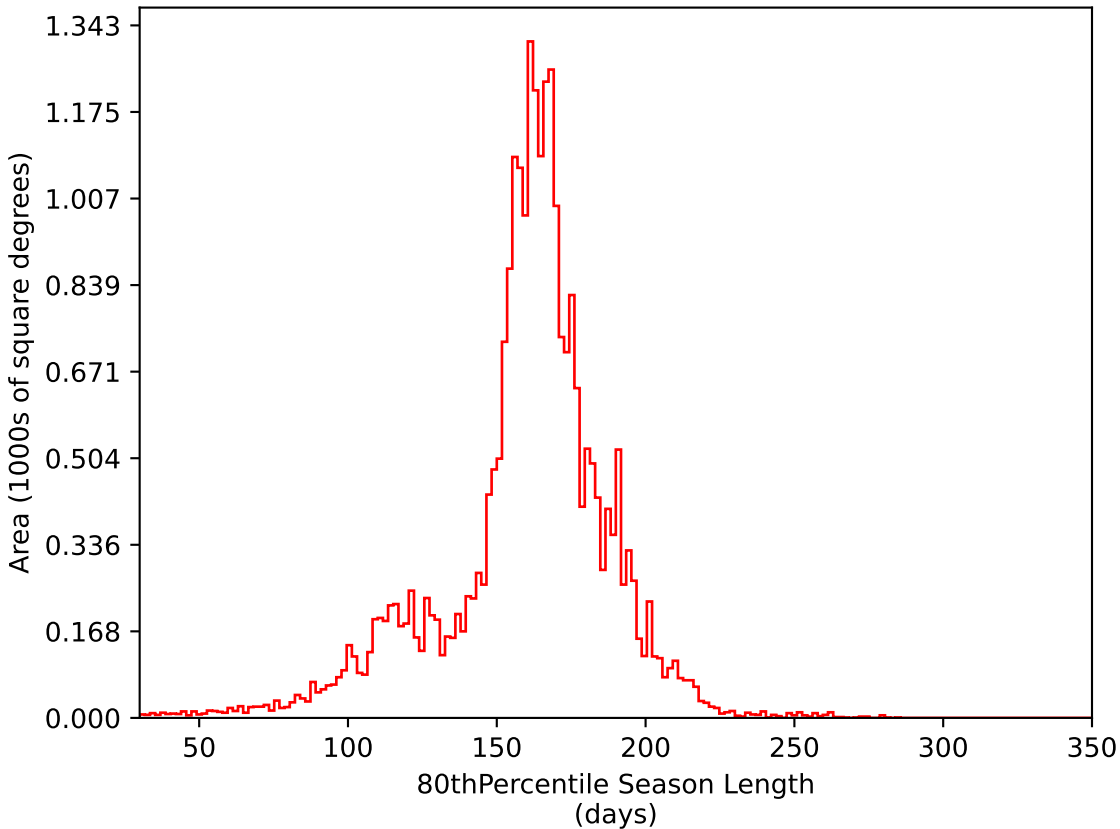
baseline_v3.3_10yrs All sky i band: 80thPercentile Season Length
