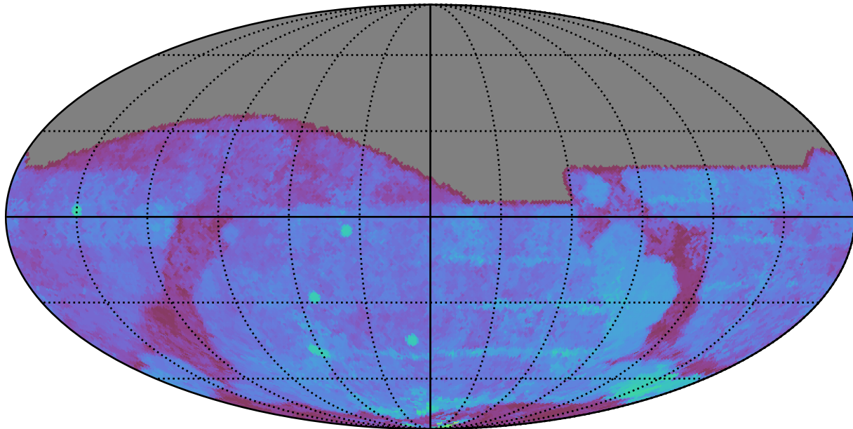
baseline_v3.3_10yrs All sky g band: 80thPercentile Season Length
