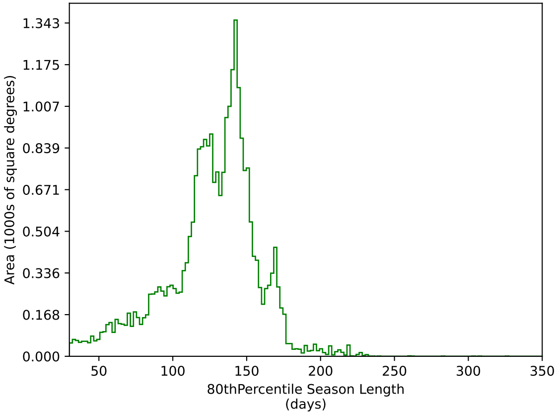
baseline_v3.3_10yrs All sky g band: 80thPercentile Season Length
