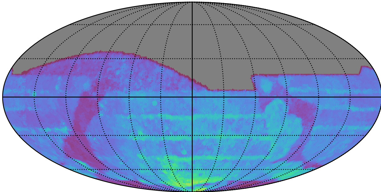
baseline_v3.3_10yrs All sky all bands: 80thPercentile Season Length
