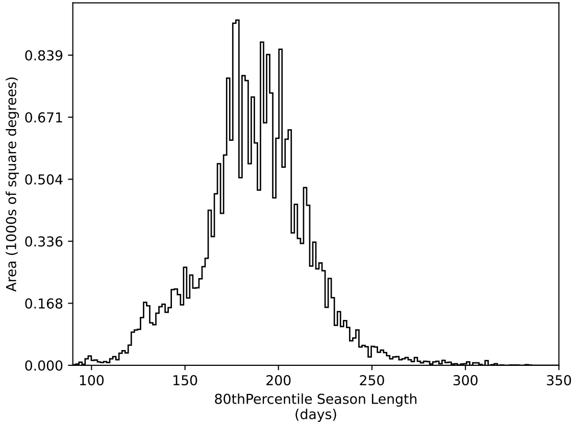
baseline_v3.3_10yrs All sky all bands: 80thPercentile Season Length
