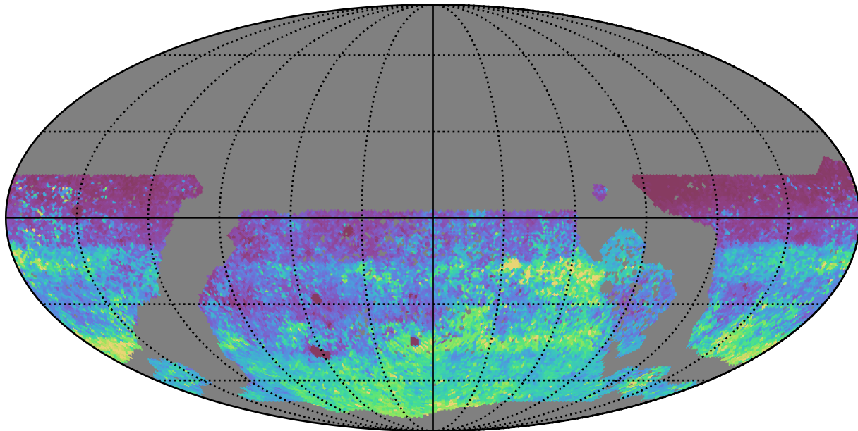
baseline_v3.3_10yrs WFD zy bands: 75th Percentile Intranight Timespan
