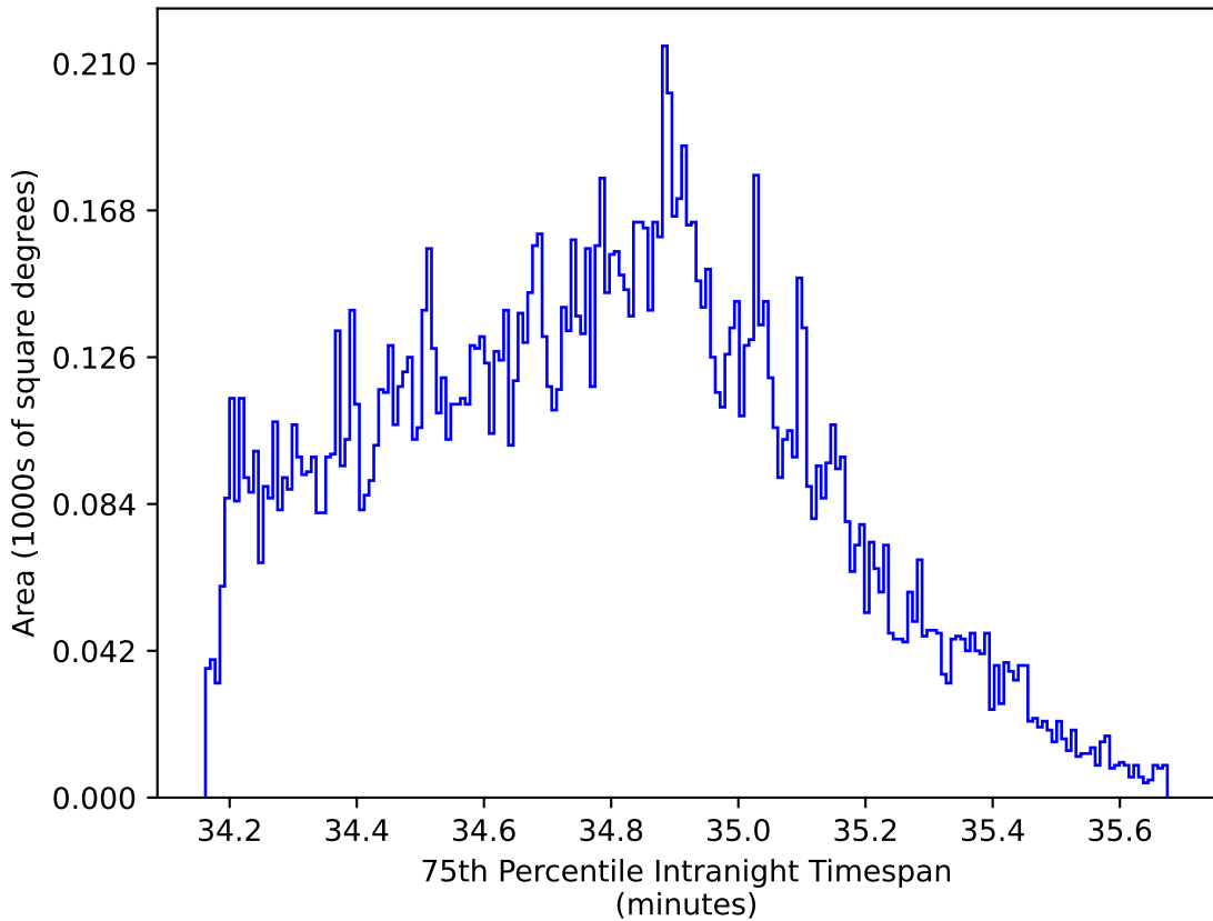
baseline_v3.3_10yrs WFD zy bands: 75th Percentile Intranight Timespan
