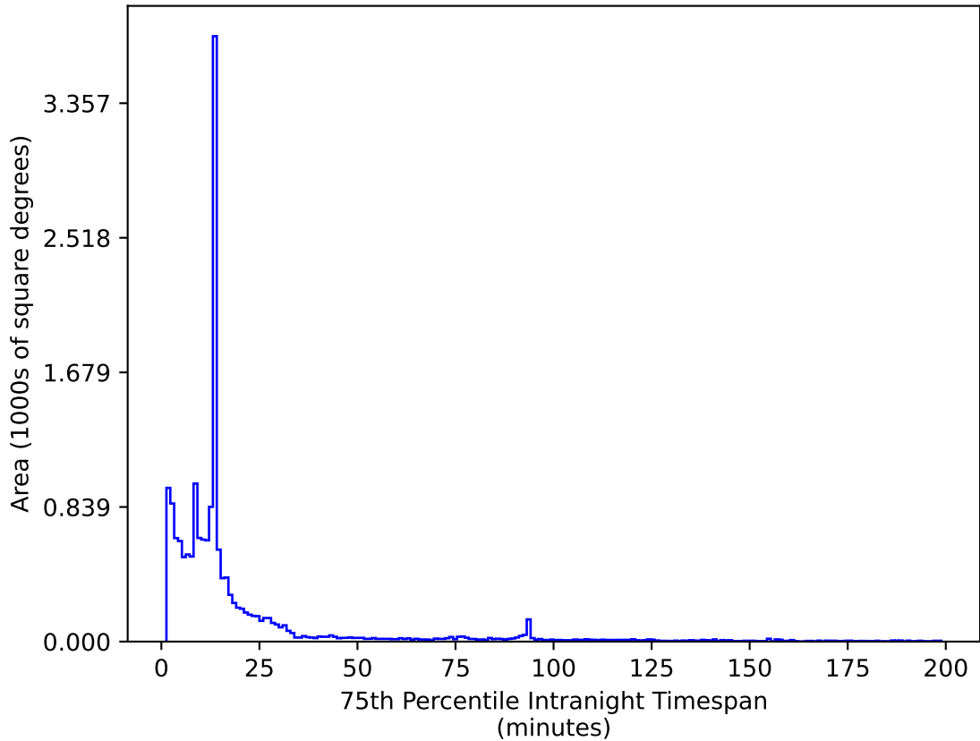
baseline_v3.3_10yrs WFD z band: 75th Percentile Intranight Timespan
