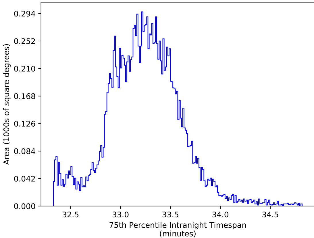
baseline_v3.3_10yrs WFD y band: 75th Percentile Intranight Timespan
